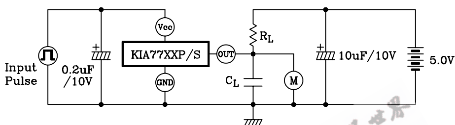
APPLICATION CIRCUIT
