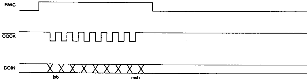
Figure 8. 1-byte command input
