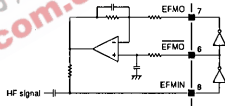
Figure 1. HF input circuit
