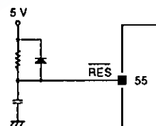
Figure 17. Power-ON reset circuit
