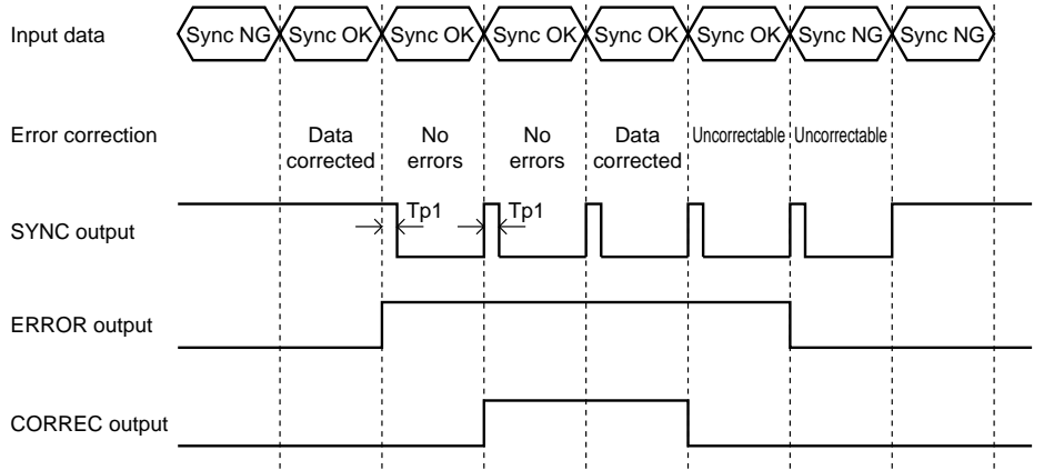
Timing 2 (mode 3, PT2 = 0)
