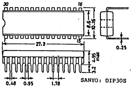
Case Outline—[3052A] unit: mm
