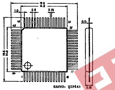
Case Outline—[3029A] unit: mm
