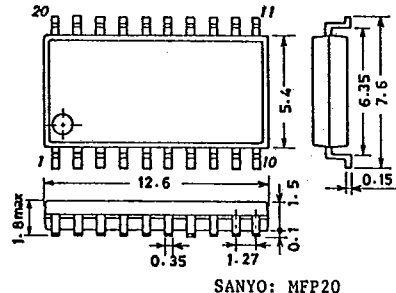
Case Outline—[3044B] unit: mm
