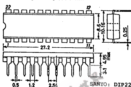
Case Outline—[3010A] unit: mm
