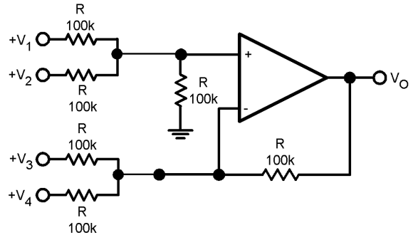
DC Summing Amplifier ( V_{IN's} \geq 0 V_{DC} and V_O \geq V_{DC} )
