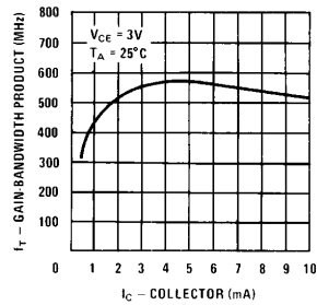
Typical Gain-Bandwidth Product vs Collector Current
