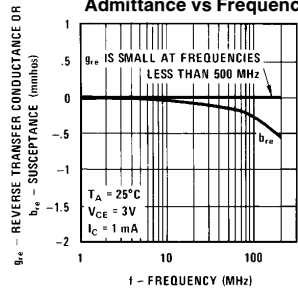
Typical Reverse Transfer Admittance vs Frequency
