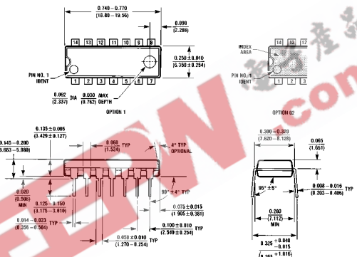
Molded Dual-In-Line Package (N) Order Number LM3046N or LM3086N NS Package Number N14A
