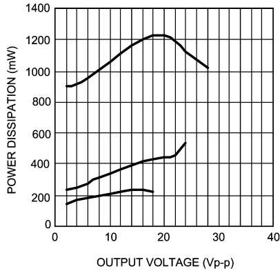
Power Dissipation vs Output Voltage V_{DD} = 3V , from top to bottom: V_1 = 15V, V_1 = 12V, V_1 = 9.6V
