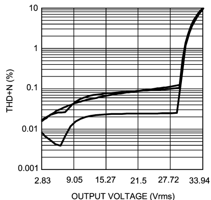
THD+N vs Output Power V_{DD} = 5V, V_1 = 15V, f = 100Hz, 1kHz, 10kHz
