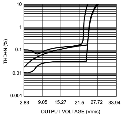
THD+N vs Output Power V_{DD} = 3V, V_1 = 12V, f = 100Hz, 1kHz, 10kHz
