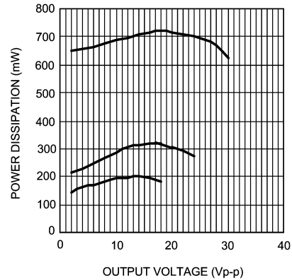
Power Dissipation vs Output Voltage V_{DD} = 5V , from top to bottom: V_1 = 15V, V_1 = 12V, V_1 = 9.6V
