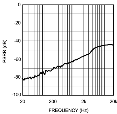
Power Supply Rejection Ratio V_{DD} = 5V
