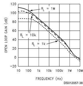
Open Loop Gain vs Load, 5V Supply
