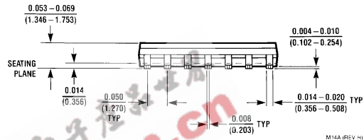
14-Pin Small Outline Package Order Number LM6144AIM or LM6144BIM NS Package Number M14A
