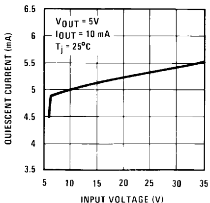
Quiescent Current
