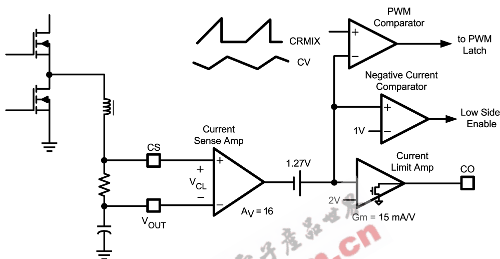
FIGURE 6. Current Sensing and Limiting
