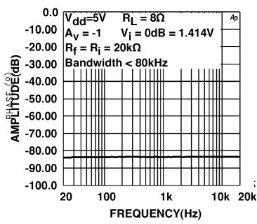
Output Attenuation in Shutdown Mode
