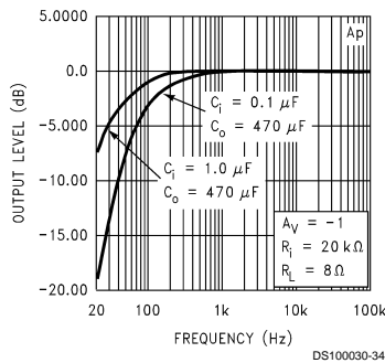
Typical Application Frequency Response
