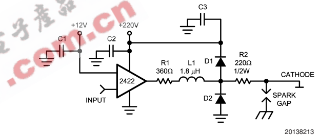
FIGURE 13. One Channel of the LM2422 with the Recommended Application Circuit
