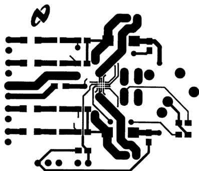
10099345 Figure 13. Recommended 20-pin micro SMD PC Board Layout: Component-Side Layout
