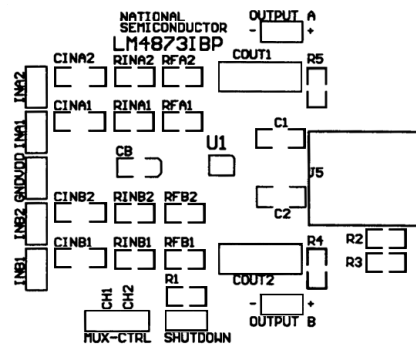
Figure 12. Recommended 20-pin micro SMD PC Board Layout: Component-Side Silkscreen
