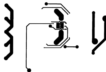
10099346 Figure 14. Recommended 20-pin micro SMD PC Board Layout: Upper Inner-Layer Layout
