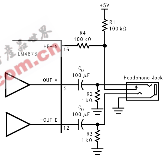
FIGURE 3. Headphone Circuit
