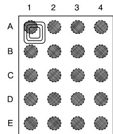
Top View (Bump-side down) Order Number LM4873IBL, LM4873ITL See NS Package Number BLA20AAB for micro SMD See NS Package Number TLA20AAA
