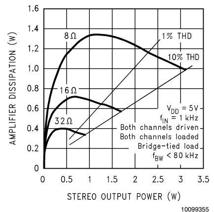
LM4873IBL Stereo Output Power vs Power Dissipation
