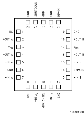
Top View Order Number LM4873LQ See NS Package Number LQA24A for Exposed-DAP LLP
