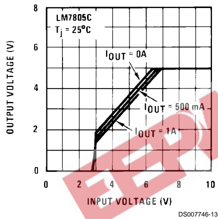
Dropout Characteristics
