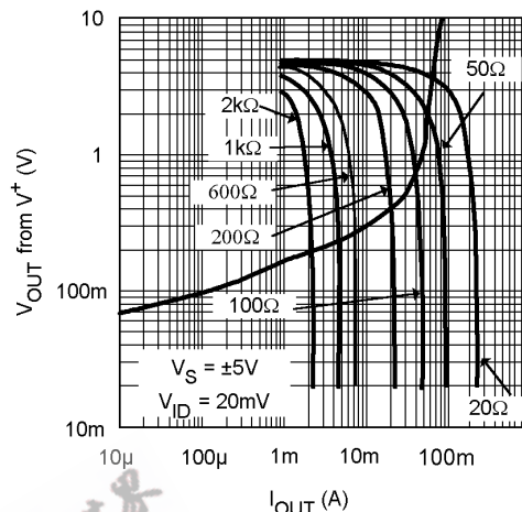
FIGURE 3. Steady State Output Sourcing Characteristics with Load Lines
