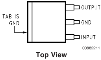
(TO-263) Surface-Mount Package
