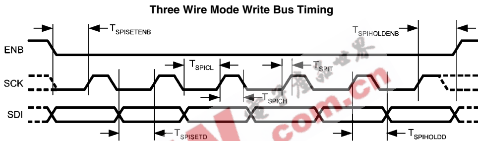
FIGURE 2. Three Wire Mode Write Bus
