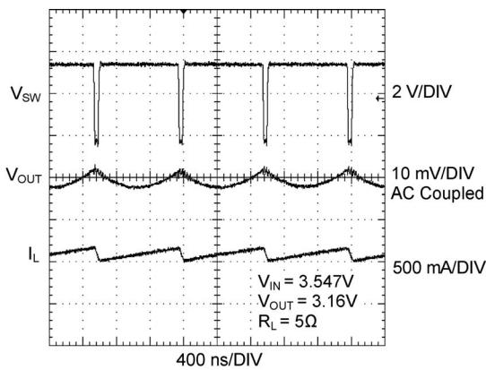
Output Voltage Ripple in Pulse Skip ( V_{IN} = 3.547V , V_{OUT} = 3.16V , R_{LOAD} = 5\Omega )
