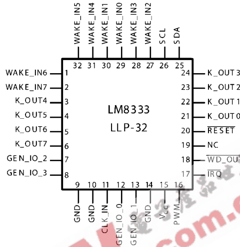
Top View Leadless Leadframe Package See NS Package Number LQA32A
