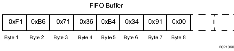
FIGURE 2. Example Event Codes Loaded in FIFO Buffer
