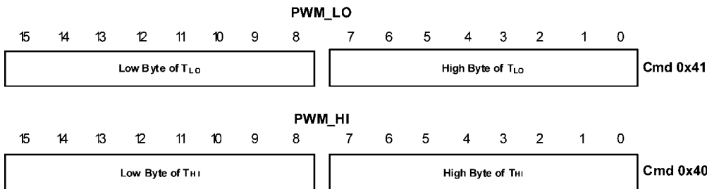
FIGURE 4. PWM Control Commands for Arbitrary Duty Cycle
