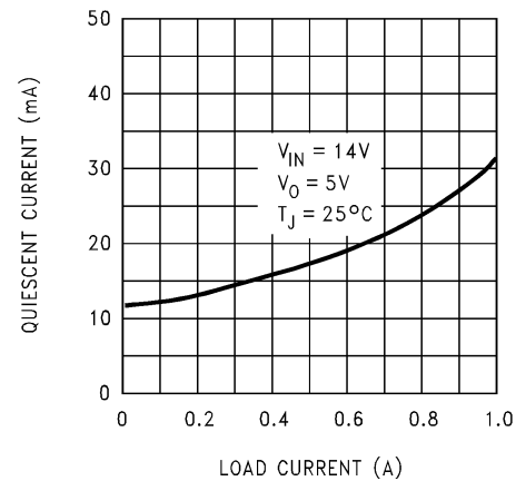
Quiescent Current
