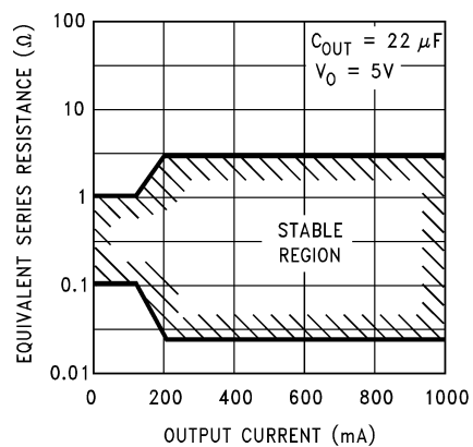
FIGURE 1. ESR Limits
