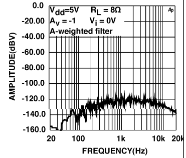
Noise Floor
