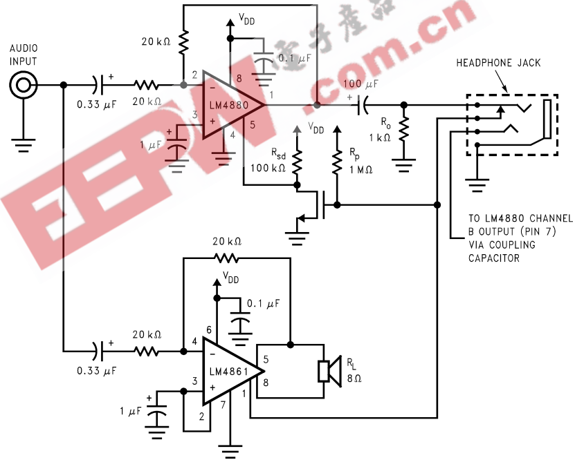
FIGURE 3. Automatic Switching Circuit
