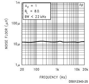
Noise Floor
