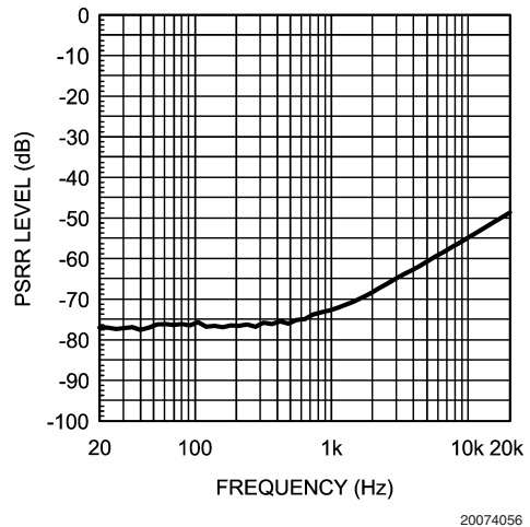
Power Supply Rejection Ratio (PSRR) vs Frequency V_{DD} = 3V, R_L = 8\Omega, \text{ input floating}
