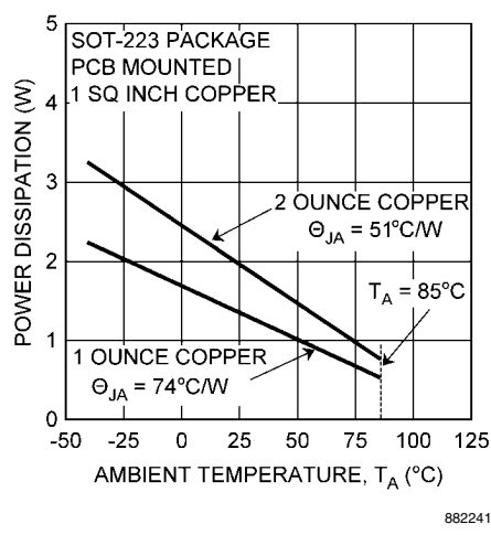
FIGURE 6. Maximum Power Dissipation vs. T_A for the SOT-223 Package
