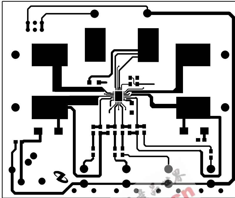
FIGURE 5. Top Layer
