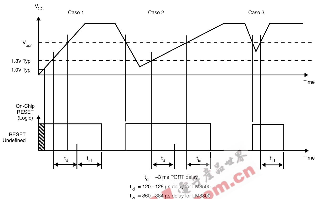
FIGURE 4. Brownout Reset Operation
