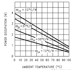
Maximum Power Dissipation (TO-263) (Note 3)
