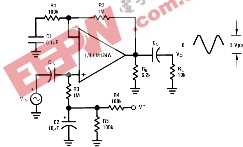
AC Coupled Non-Inverting Amplifier
