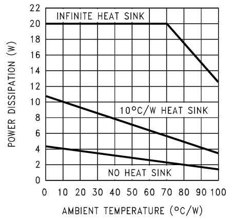
Maximum Power Dissipation (TO-3)
