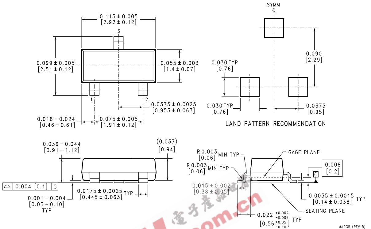
SOT-23 Molded Small Outline Transistor Package (M3) Order Number LM60BIM3 or LM60CIM3 NS Package Number MA03B
