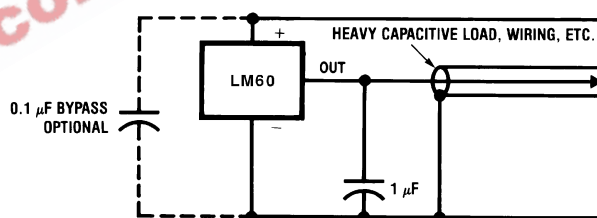
FIGURE 5. LM60 with Filter for Noisy Environment
