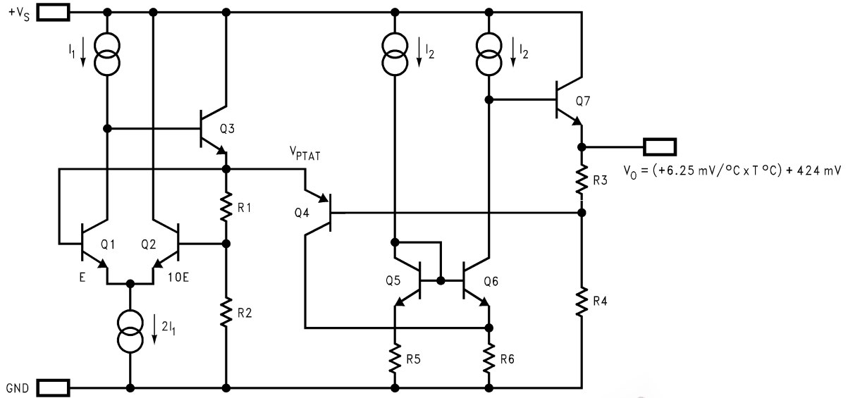
FIGURE 6. Simplified Schematic
