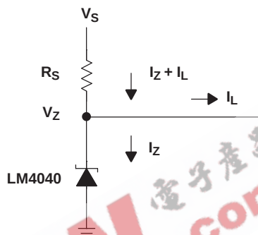
Figure 9. Shunt Regulator
