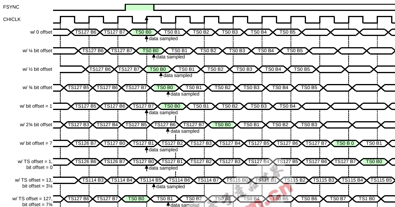
Figure 5-13. Typical Receive CHI Timing with 8.192 Mbits/s Data and 8.192 MHz CHICLK
