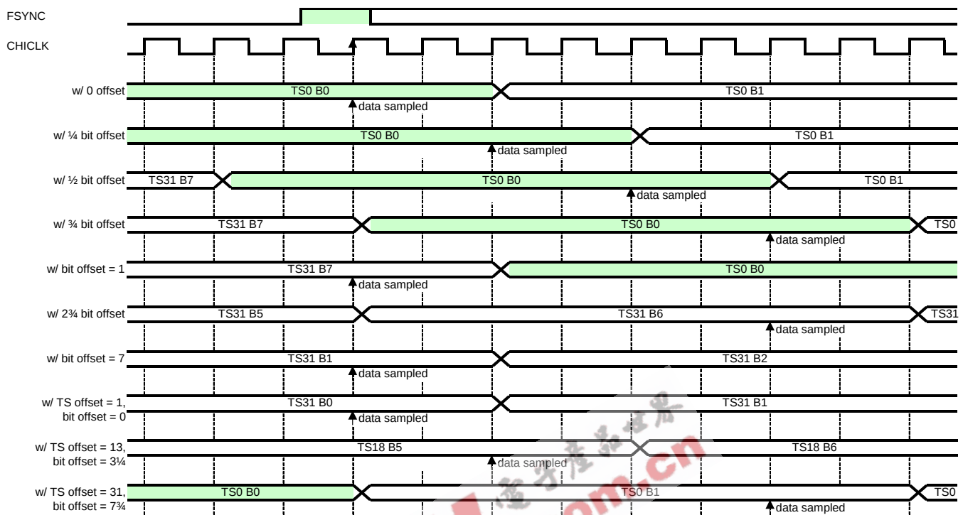
Figure 5-11. Typical Receive CHI Timing with 2.048 Mbits/s Data and 16.384 MHz CHICLK
