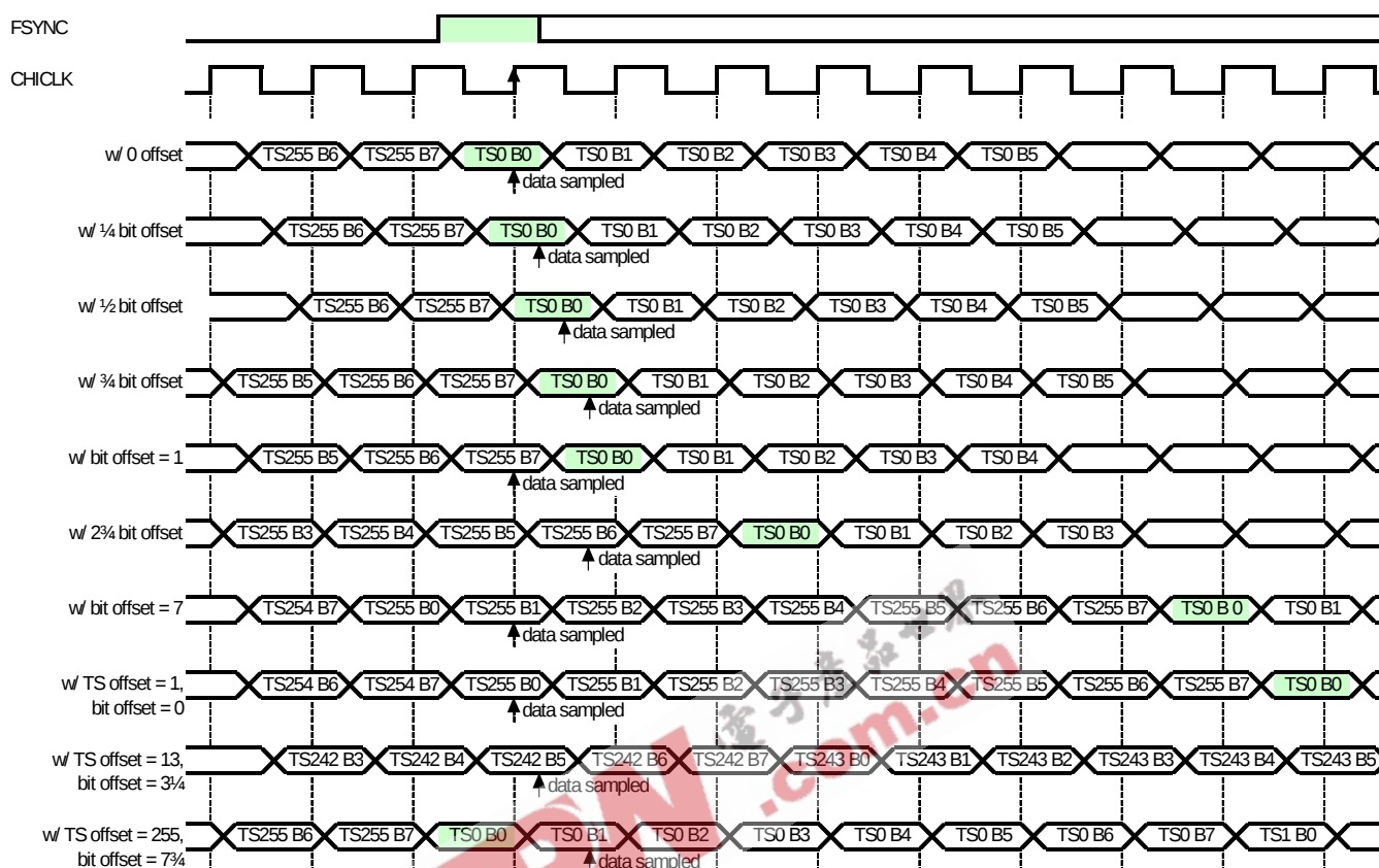
Figure 5-5. Typical Receive CHI Timing with 16.384 Mbits/s Data and 16.384 MHz CHICLK
