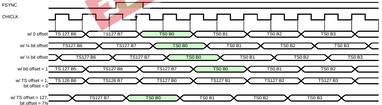
Figure 5-8. Transmit CHI Timing with 8.192 Mbits/s Data and 16.384 MHz CHICLK
