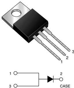
TO-220AB
