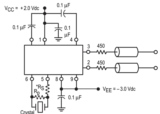
Figure 7. AC Test Circuit – Sine Wave Output
