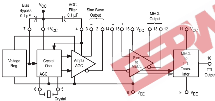
Figure 1. Block Diagram
