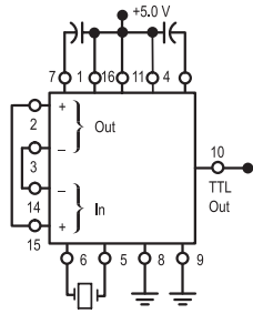
Figure 3. MTTTL Output
