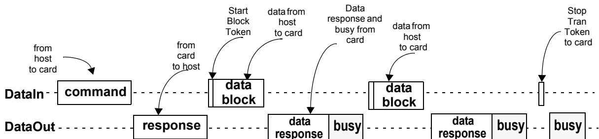
Figure 7-6 : SPI Multiple Block Write Operation
