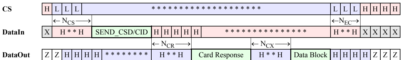
Figure 7-21 : SPI Read CSD and CID Registers
