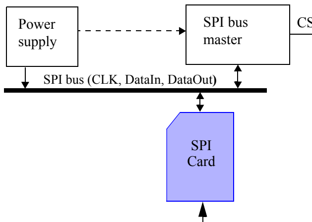
Figure 5-2 : MultiMediaCard Bus System
