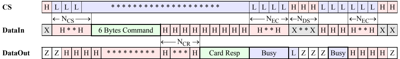
Figure 7-16 : SPI Command/Response Transaction, Card Is Busy
