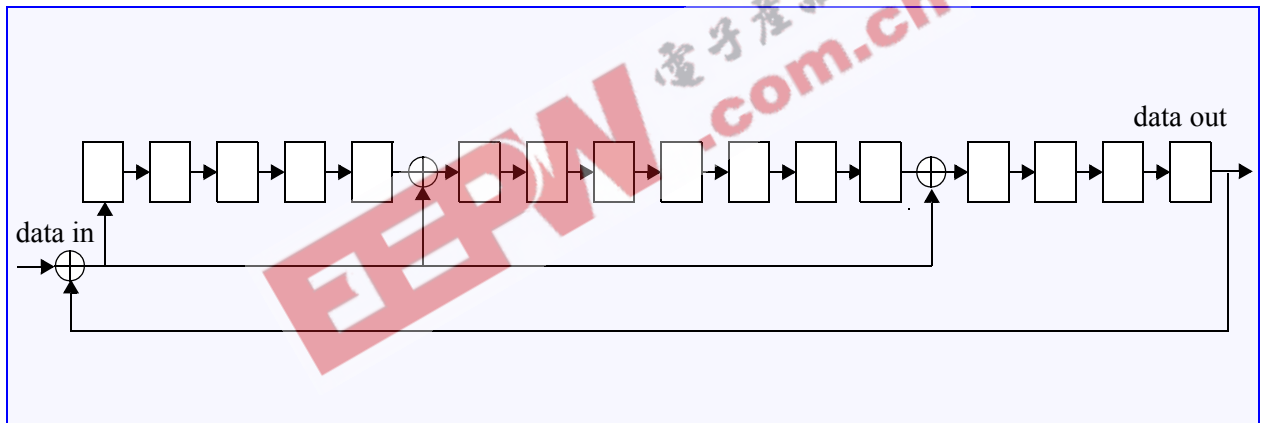
Figure 6-4 : CRC16 Generator/Checker
