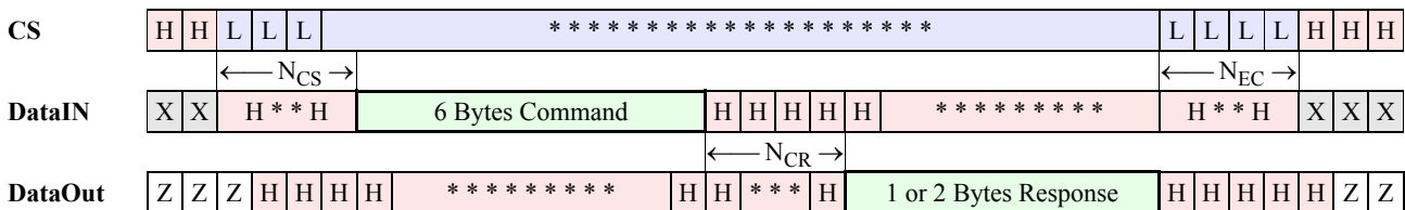
Figure 7-15 : SPI Command/Response Transaction, Card Is Ready
