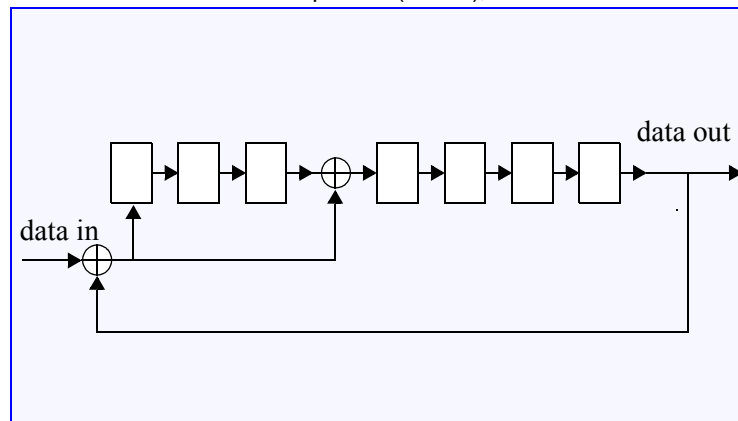
Figure 6-3 : CRC7 Generator/Checker
