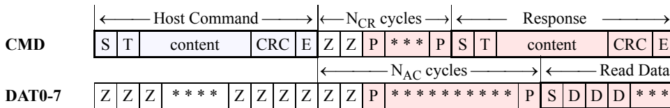
Figure 6-12 : Single Block Read Timing
