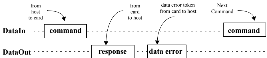
Figure 7-4 : SPI Read Operation - Data Error
