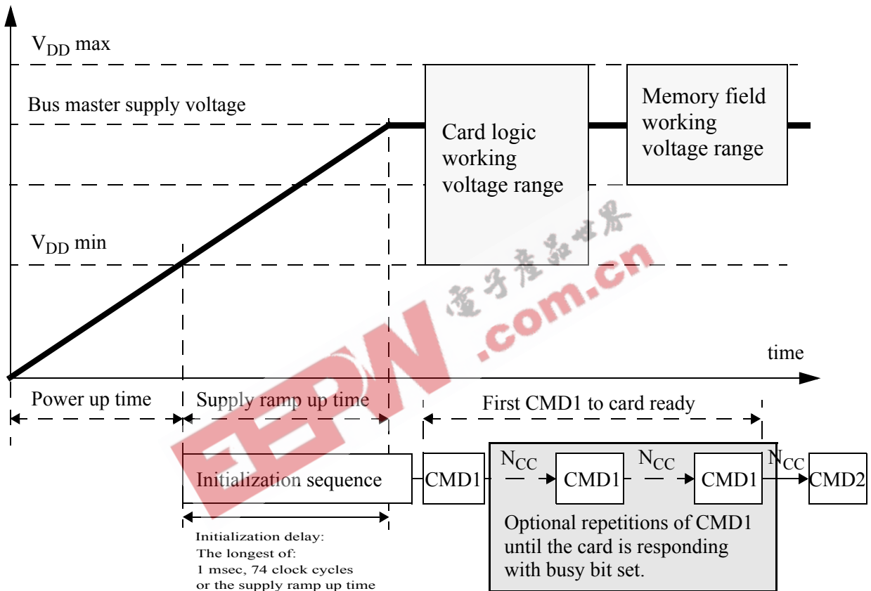
Figure 5-3 : Power-up Diagram
