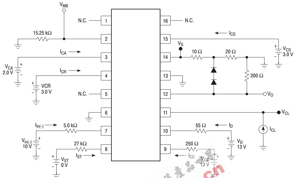
Figure 2. Test Circuit
