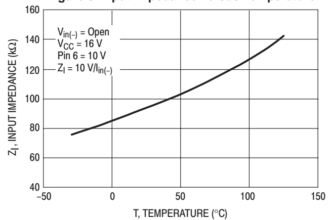
Figure 6. Input Impedance versus Temperature
