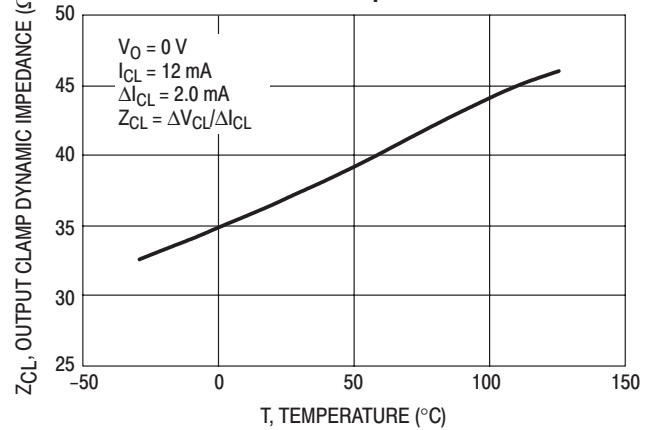
Figure 8. Output Clamp Dynamic Impedance versus Temperature
