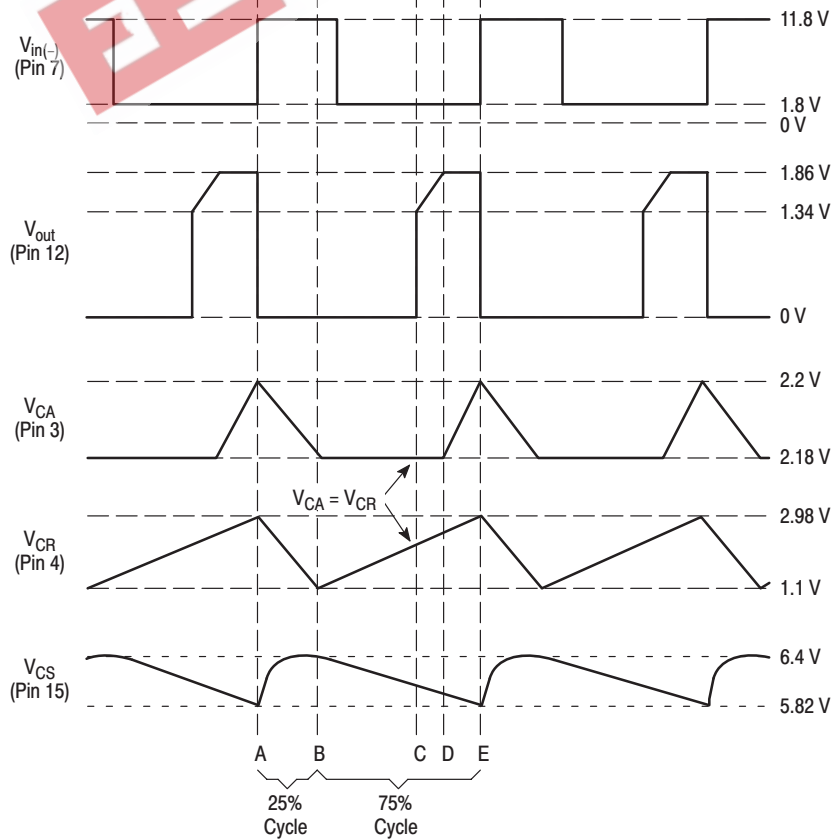
Figure 14. Run Mode 900 RPM (Frequency: 30 Hz @ 10 ms)
