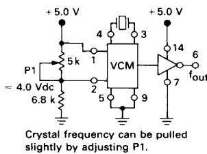
FIGURE 3 — VOLTAGE-CONTROLLED MULTIVIBRATOR
