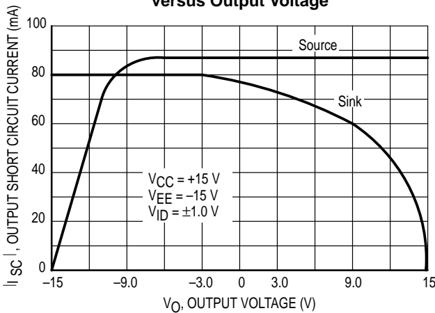
Figure 13. Output Short Circuit Current versus Output Voltage
