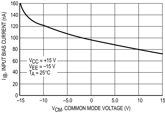
Figure 3. Input Bias Current versus Common Mode Voltage
