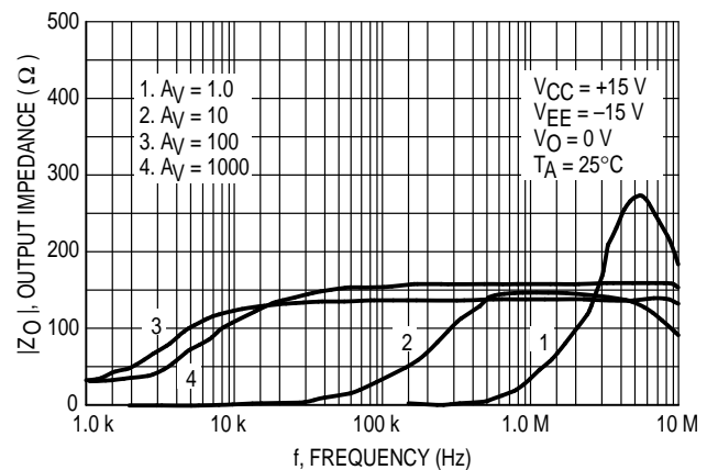
Figure 26. Output Impedance versus Frequency
