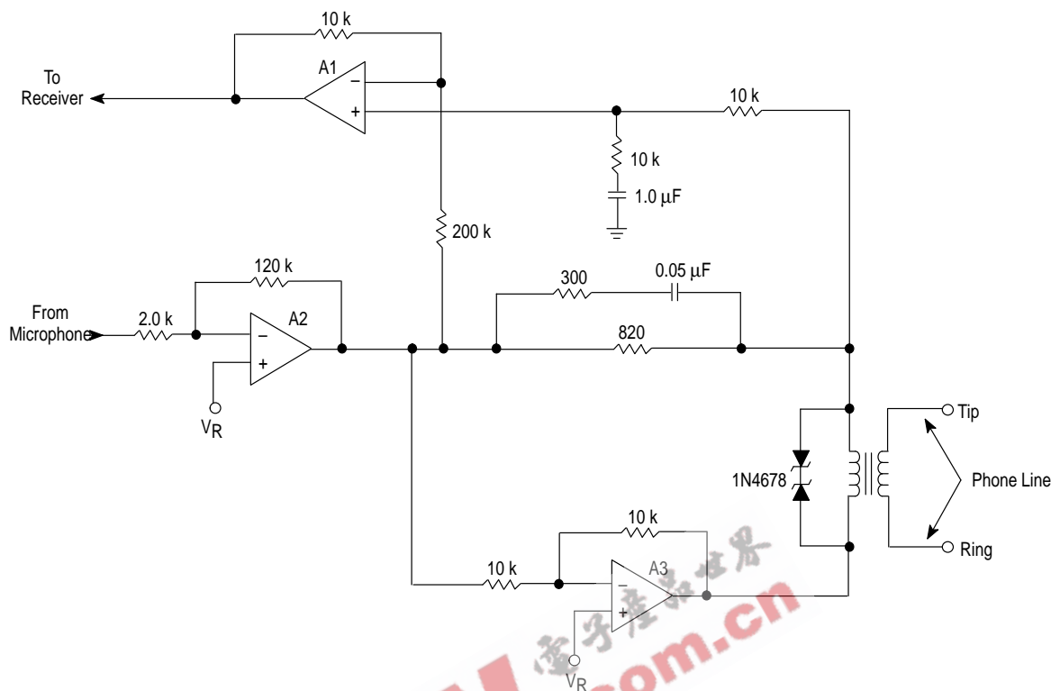
Figure 33. Telephone Line Interface Circuit
