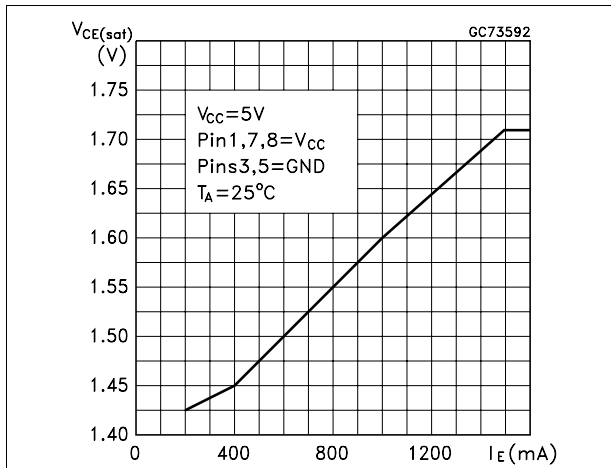
Figure 3. Emitter follower configuration output saturation voltage vs emitter current
