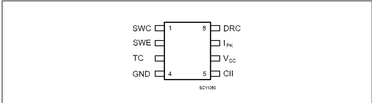
Figure 2. Pin connections
