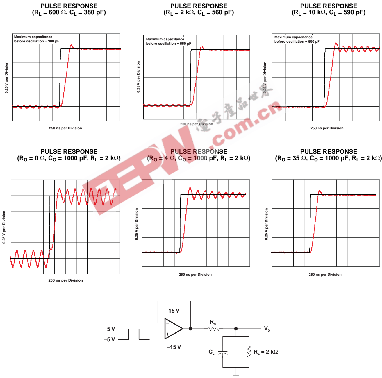
Figure 2. Output Characteristics
