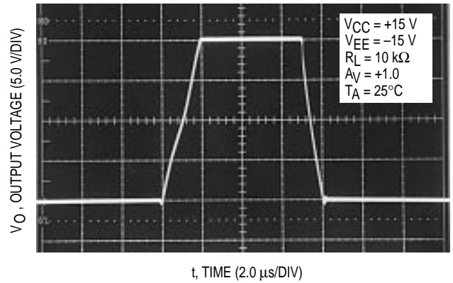
Figure 28. Transient Response
