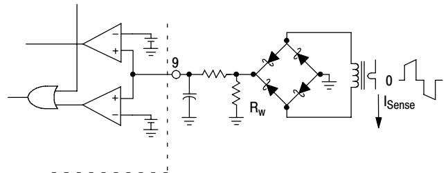
Figure 28. Primary or Secondary Side Current Sensing
