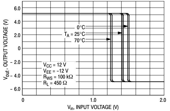
Figure 4. Input/Output Characteristics versus Temperature
