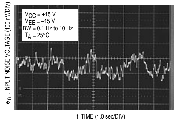
Figure 33. Low Frequency Noise Voltage versus Time
