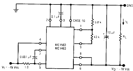
FIGURE 6 - LOAD REGULATION
