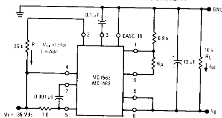
FIGURE 8 - SHUTDOWN CURRENT
