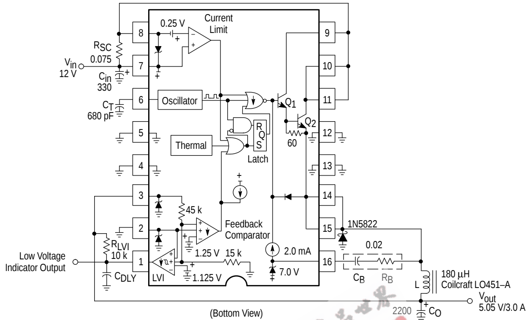
Figure 20. Step-Down Converter
