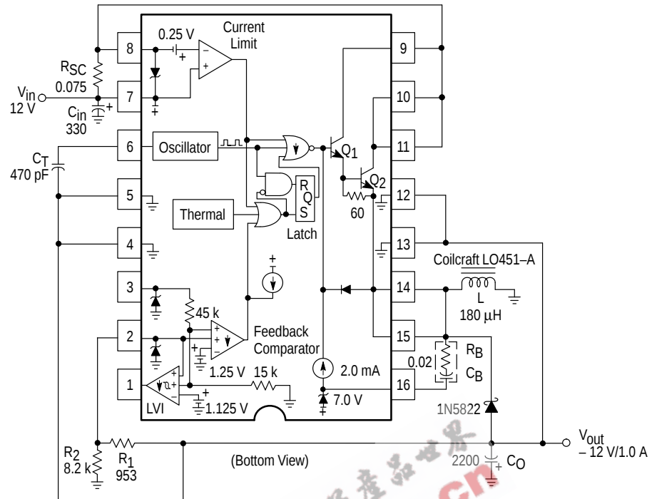
Figure 24. Voltage-Inverting Converter
