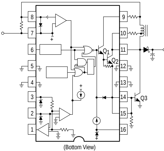
Figure 23B. External PNP Saturated Switch
