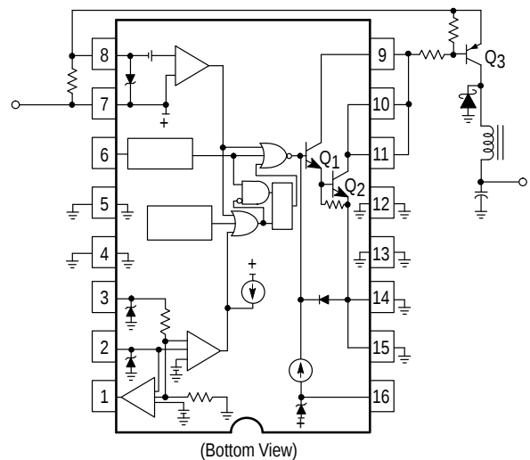
Figure 21B. External PNP Saturated Switch
