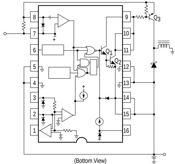
Figure 25B. External PNP Saturated Switch
