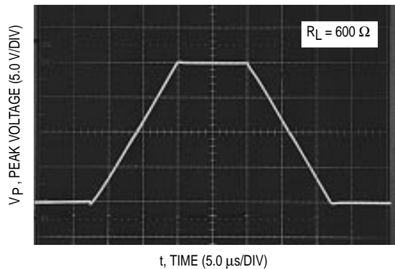
Figure 36. Awakemode Large Signal Transient Response
