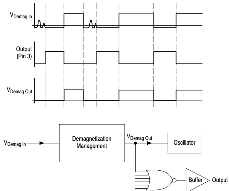
Figure 29. Demagnetization
