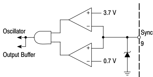
Figure 37. Synchronization
