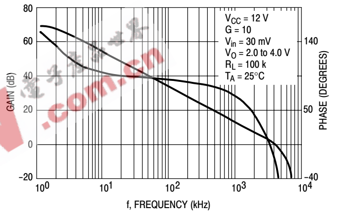
Figure 11. Error Amplifier Gain and Phase versus Frequency
