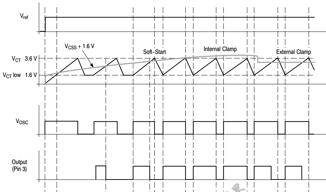
Figure 32. Soft-Start & D_{max}
