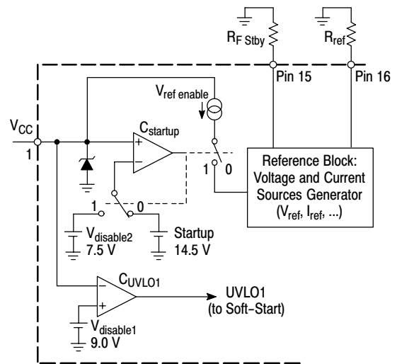
Figure 48. VCC Management
