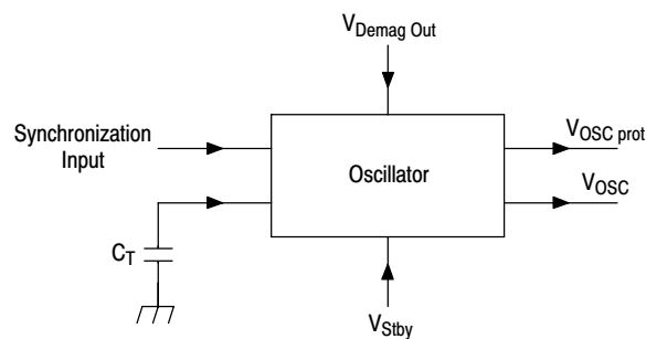
Figure 31. Oscillator
