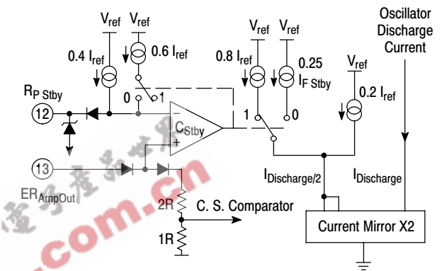
Figure 41. Standby
