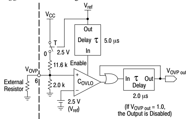
Figure 47. Overvoltage Protection
