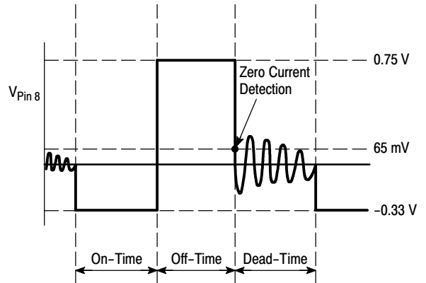
Figure 38. Demagnetization Detection
