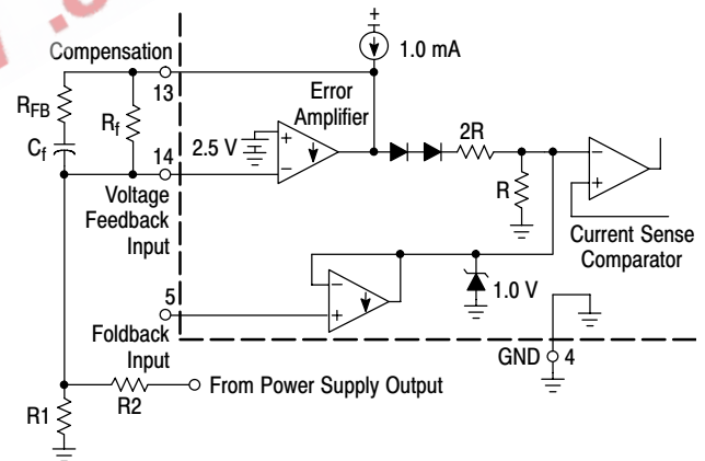
Figure 33. Error Amplifier Compensation
