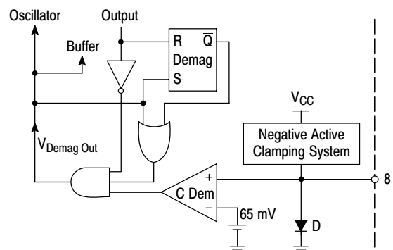
Figure 39. Demagnetization Block
